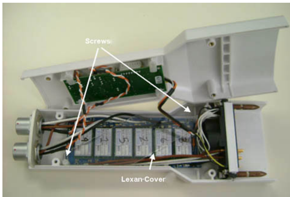
Illustration 3-4: Quick Disconnect (QD) Assembly - Two Screws and Lexan Cover
