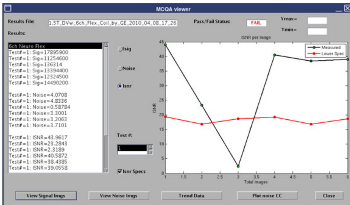
Illustration 4-4: Loss of Signal on Channel 3
