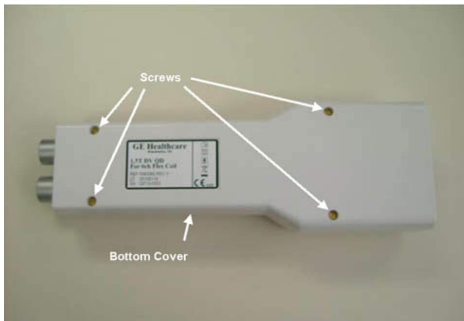
Illustration 3-2: QD Assembly - Four Screws and Bottom Cover
