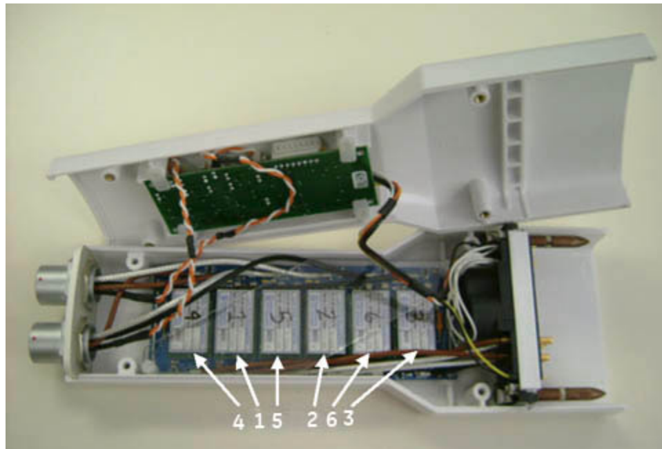
Illustration 3-7: Quick Disconnect - Preamp Locations for 1.5T and 3.0T
