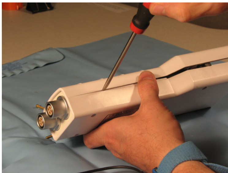
Illustration 3-3: Separating Housing on QD Assembly
