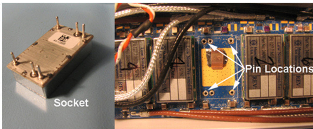
Illustration 3-6: Socket and Pin Locations on the Pre-Amp
