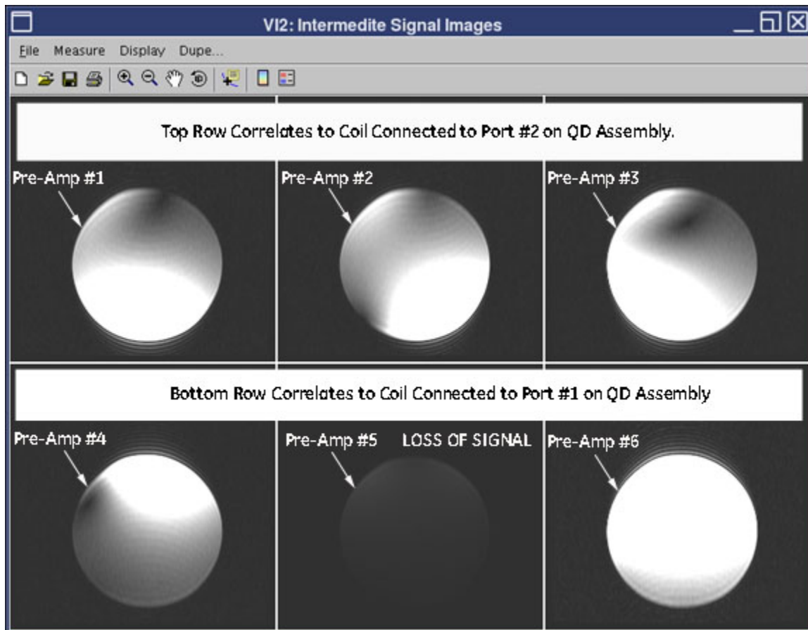
Illustration 4-1: Loss of Signal on Channel 5
