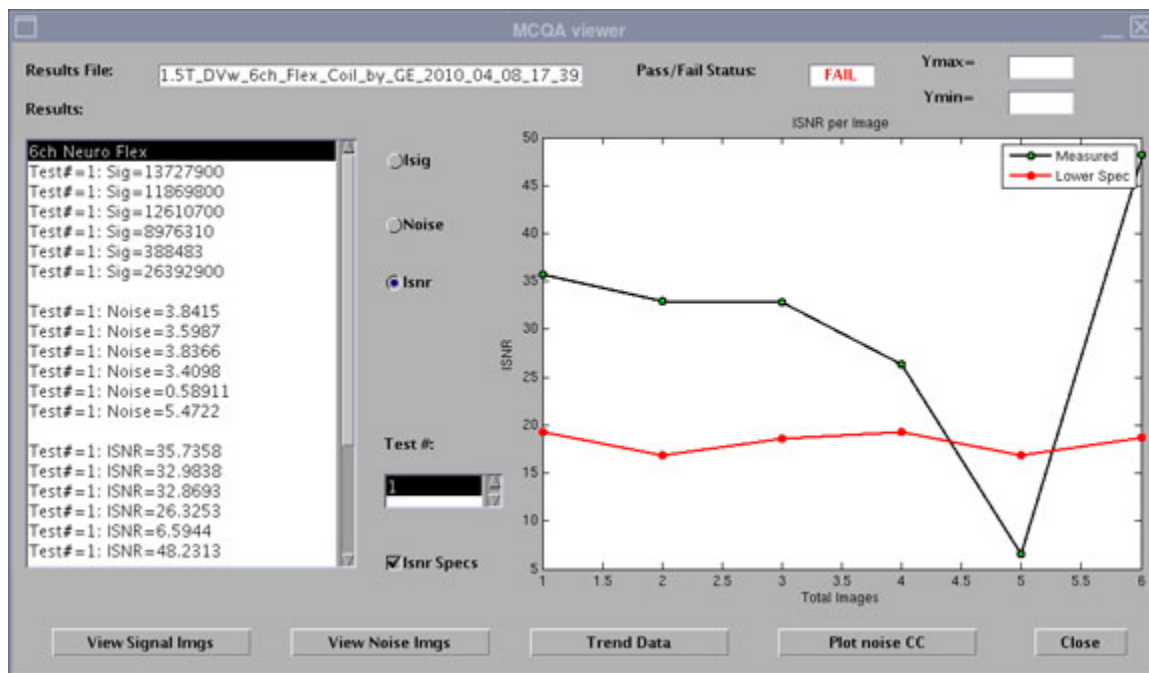
Illustration 4-2: Loss of Signal on Channel 5
